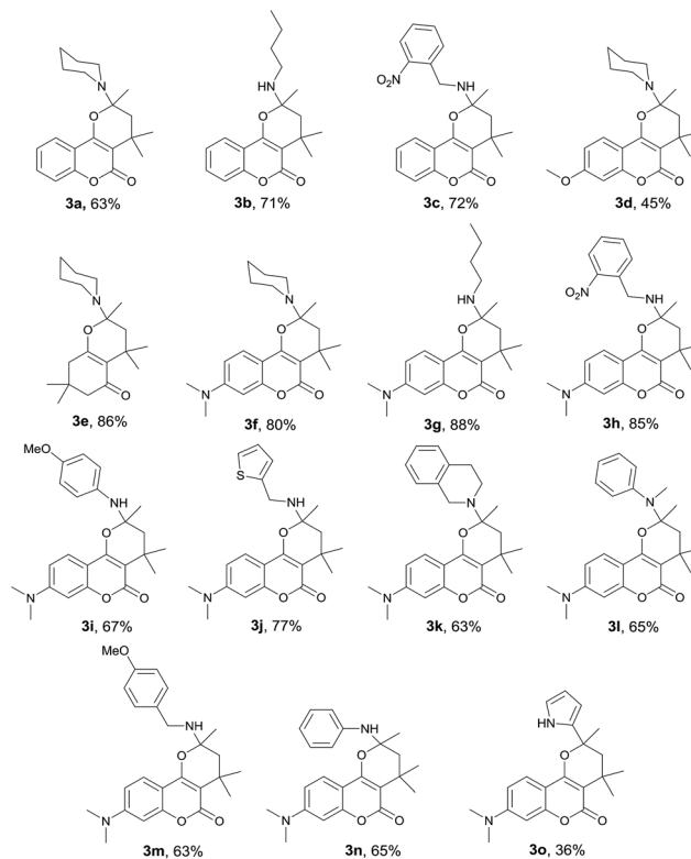
Fig. 2 Structures and yields of prepared pyranocoumarins 3a–o .
