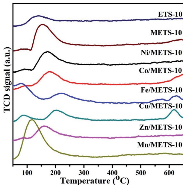
Fig. 2 \text{CO}_2 -TPD profiles of ETS-10, METS-10 and series of transition metals loaded METS-10 samples.
