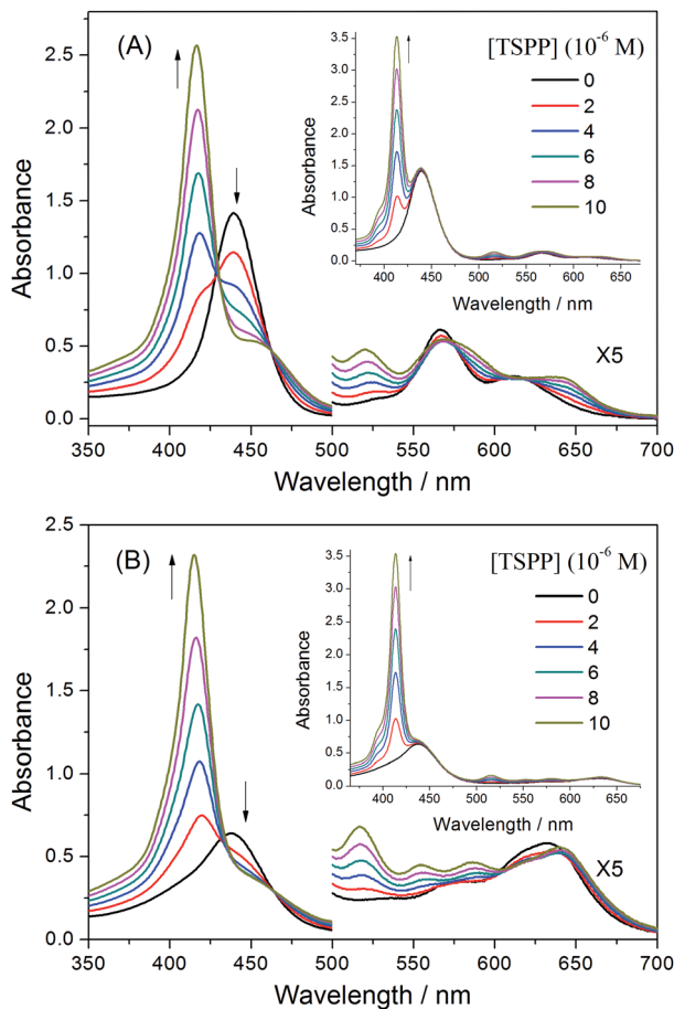
Fig. 8 UV-vis spectra of (A) P-D and (B) P-W at 2 \times 10^{-4} g mL ^{-1} with added TSPP concentrations of 0, 2 \times 10^{-6}, 4 \times 10^{-6}, 6 \times 10^{-6}, 8 \times 10^{-6}, 1 \times 10^{-5} mol L ^{-1} in water. Insets (A) and (B) show the sum of absorption spectra of (A) P-D and (B) P-W and TSPP.
