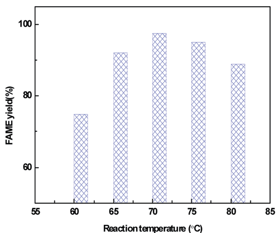
Fig. 8 Effect of reaction temperature on the FAME yield over the \text{CeO}_2 @CaO-60 catalyst.
