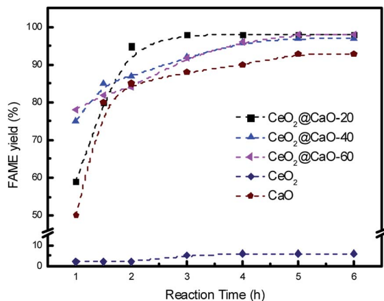
Fig. 7 Effect of reaction time on the FAME yield over the \text{CeO}_2 @CaO catalysts.
