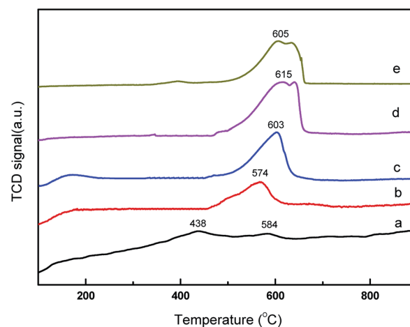
Fig. 2 \text{CO}_2 -TPD analysis of the \text{CeO}_2@\text{CaO} catalysts (a): \text{CeO}_2 , (b): \text{CeO}_2@\text{CaO} -20, (c): \text{CeO}_2@\text{CaO} -40, (d): \text{CeO}_2@\text{CaO} -60, (e): \text{CaO} .
