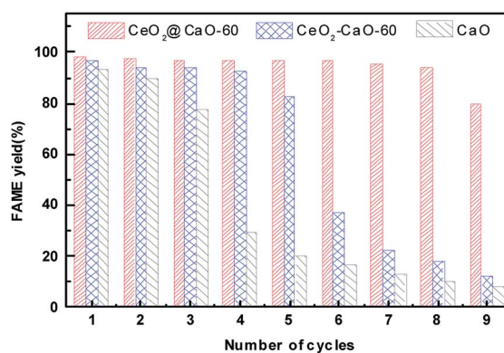
Fig. 10 The stability test of the CaO, \text{CeO}_2 @CaO-60 and \text{CeO}_2 -CaO-60 catalysts.
