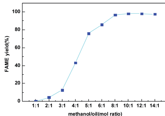
Fig. 9 Effect of methanol to oil mol ratio on the FAME yield over the \text{CeO}_2 @CaO-60 catalyst.
