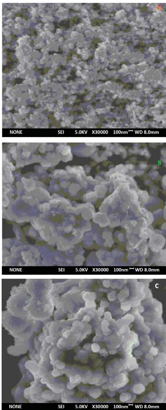
Fig. 1 SEM images of Fe 3 O 4 (A), Fe 3 O 4 @SiO 2 (B) and UMCA (C).
