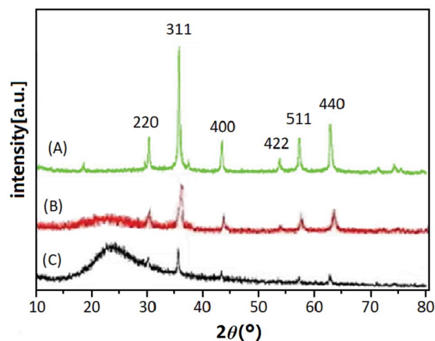
Fig. 2 XRD patterns of Fe 3 O 4 (A), Fe 3 O 4 @SiO 2 (B) and UMCA (C).
