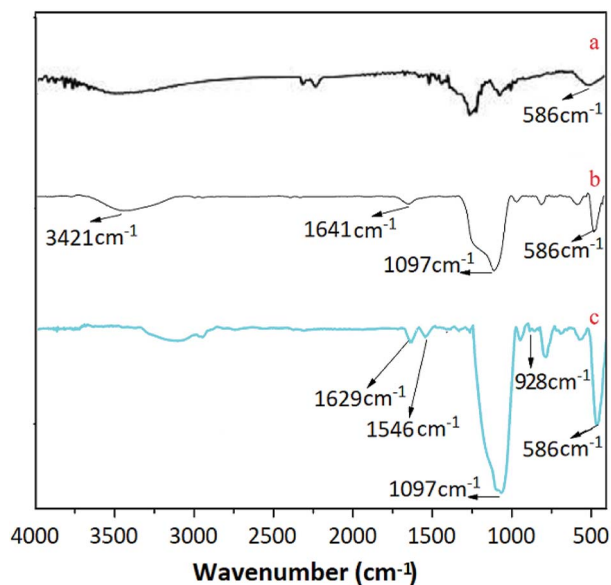
Fig. 3 FTIR spectra of Fe 3 O 4 (a), Fe 3 O 4 @SiO 2 (b) and UMCA (c).
