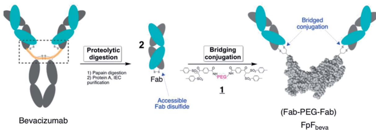
Fig. 1 Synthetic route to make FpF_{beva} from bevacizumab. Fab_{beva} was obtained by papain enzymatic digestion of bevacizumab and purified using protein A and ion-exchange chromatography (IEC). The accessible interchange disulfide in the Fab_{beva} was then reduced by DTT and conjugated with PEG-di(bis-sulfone) 1 . Each bis-sulfone moiety in reagent 1 undergoes site-specific conjugation with the two cysteine thiols from a disulfide bond by a sequence of addition–elimination reactions to insert a stable 3-carbon methylene bridge between the two thiols of the original disulfide bond.
