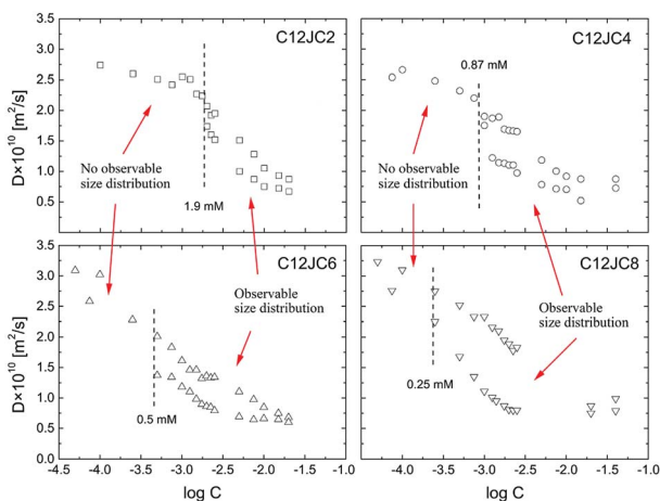
Fig. 5 The concentration dependence of the self-diffusion coefficients D obtained from BDOSY 2D displays and distribution of diffusion coefficients for C12JC2–C12JC8 gemini surfactants in D_2O .
