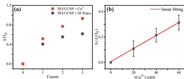
Fig. 5 (a) Luminescence quenching of the single particle fluorescent probe with 20\ \text{nM} copper ion solution and water solvent, respectively (b) linear data fitting on the degree of luminescence quenching of the single particle fluorescent probe with the concentration of copper ions after taking off the solvent contribution.
