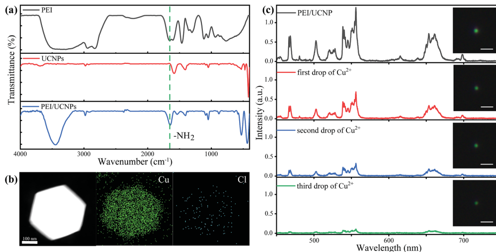
Fig. 4 (a) Fourier transform infrared spectra of the PEI, bare and PEI modified \text{NaYF}_4:\text{Yb}^{3+}/\text{Er}^{3+}/\text{Zn}^{2+} nanoparticles, (b) the distribution of copper and chloride ions on single particle fluorescent probe after the addition of 1\ \mu\text{M} \text{CuCl}_2 solution to the particle, (c) emission spectra and corresponding microscopic images of the single particle probe before and after adding copper ion solution on it, and the scale bars are 2\ \mu\text{m} .
