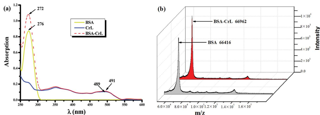
Fig. 1 (a) UV-visible spectra of 20 \mu M BSA (yellow solid line), 20 \mu M CrL complex (blue solid line) and 20 \mu M BSA-CrL hybrid (red dashed line) in 0.05 M PBS buffer pH 7.45; (b) ESI-TOF MS spectrum of BSA and BSA-CrL.
