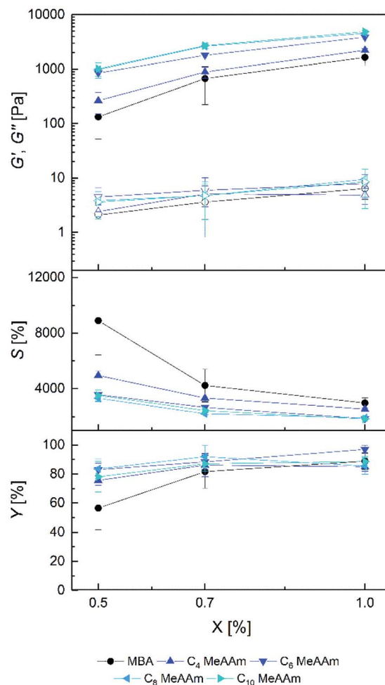
Fig. 3 Storage modulus G' (filled symbols), loss modulus G'' (open symbols), equilibrium degree of swelling S and gel yield Y of prepared PDMAAm hydrogels with different ratios of C 4 – C 10 MeAAm cross-linker ( X ). Standard deviation is given as error bars ( n = 9).
