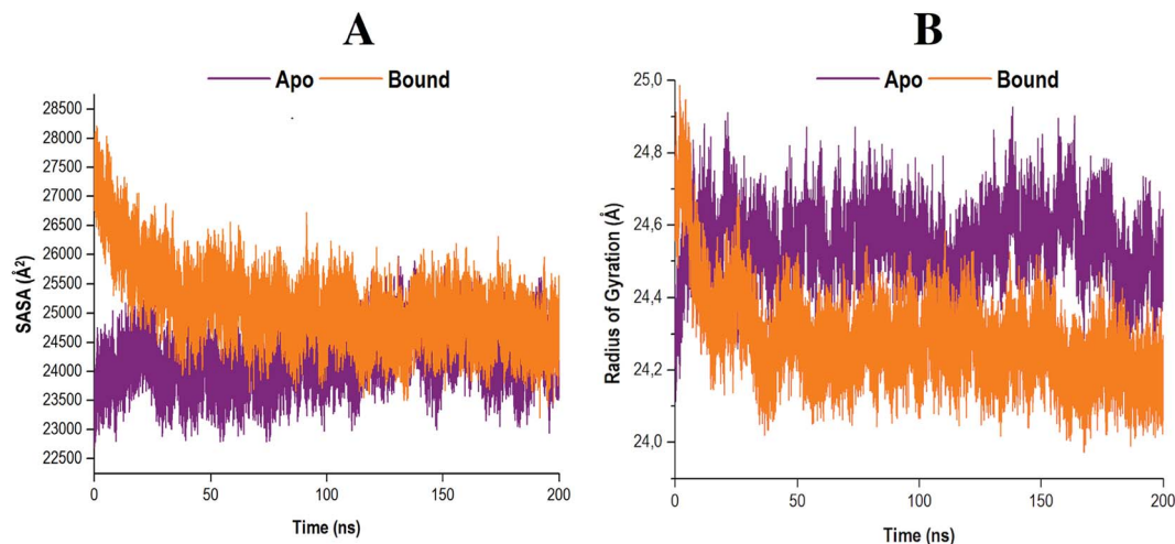
Fig. 8 (A) Solvent accessible surface area of apo and compound 47 bound RdRp. (B) Radiuses of gyration of both systems were measured over a 200 ns simulation. Data obtained were represented as a plot displaying the differences arising in radius deviation between the apo and covalent systems.
