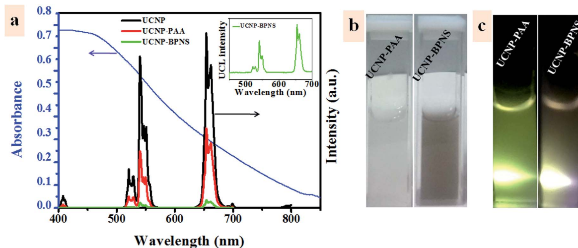
Fig. 3 (a) Upconversion emission spectra of UCNPs, UCNPs-PAA and UCNPs-BPNS, with the visible absorption spectrum of BPNS (blue line). The inset shows the magnified upconversion emission spectrum of UCNPs-BPNS nanocomposite. (b) The bright-field photographs of UCNPs-PAA and UCNPs-BPNS in H 2 O (from left to right) and (c) their corresponding upconversion emission photographs when being excited with 980 nm laser (0.5 W cm -2 ), respectively.
