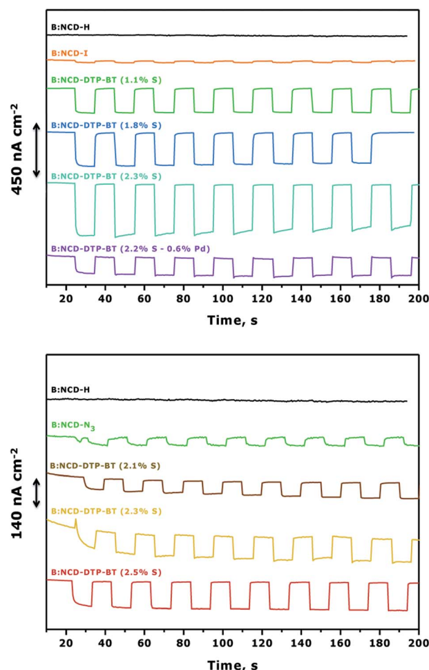
Fig. 6 Photocurrent densities (nA cm -2 ) of H-terminated (B:NCD-H), iodophenyl (B:NCD-I), azidophenyl (B:NCD-N 3 ) and DTP-BT functionalized (B:NCD-DTP-BT) diamond electrodes in a 5 mM methyl viologen solution (in 0.1 M Na 2 SO 4 ) under white light illumination (90 mW cm -2 ; simulated AM 1.5G solar spectrum, 10 s 1 : 1 dark/light interval) at a bias of -0.2 V. Surface functionalization was performed via Sonogashira cross-coupling (top) and CuAAC (bottom).
