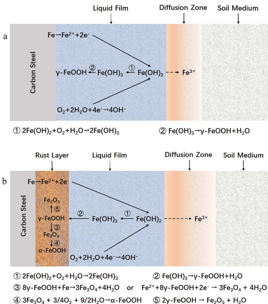
Fig. 9 Corrosion products and the iron ion diffusion models of carbon steel, (a) the initial stage in corrosion processes and (b) development stage associated with the supplement of oxygen.
