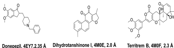
Fig. 14 Cocystal ligands structure with PDB id and resolution.
