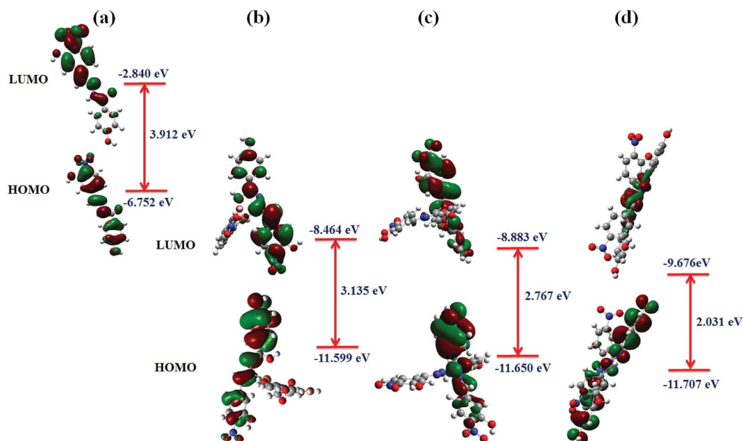
Fig. 7 Calculated frontier molecular orbitals of 3-HNHBH and the corresponding HOMO and LUMO orbital energies (a) before, and after complexation with (b) \text{Cu(II)} , (c) \text{Zn(II)} and (d) \text{Ni(II)} metal ions.
