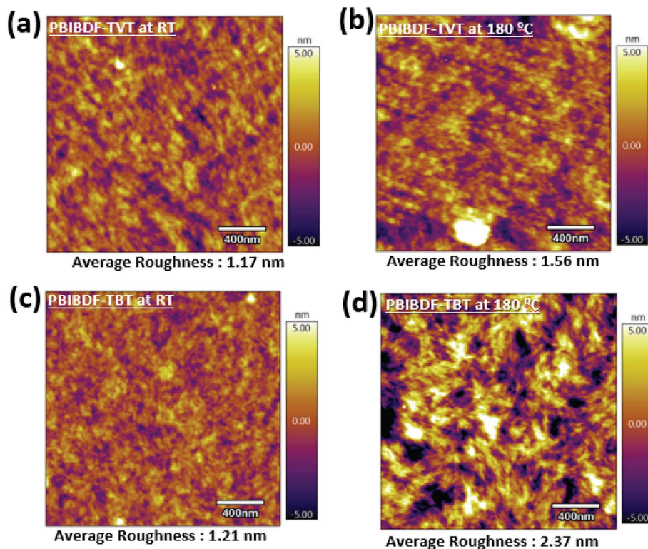
Fig. 10 AFM Images (2 \mu\text{m} by 2 \mu\text{m} ) of (a) PBIBDF-TV at room temperature and (b) at 180 °C, (c) PBIBDF-TBT at room temperature and (d) at 180 °C.
