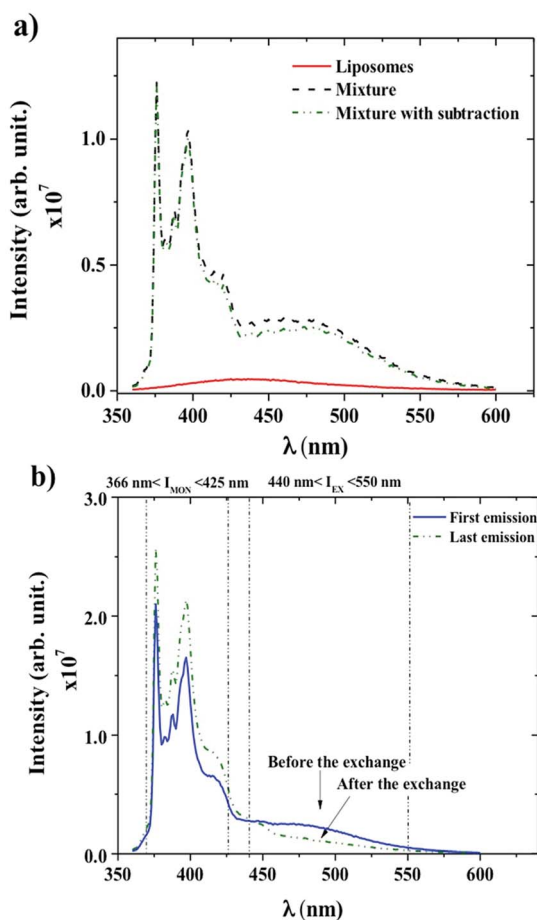
Fig. 4 (a) Emission spectra of liposomes suspension at a concentration of 25 \text{ mg mL}^{-1} and emission spectra of PyC 18 in an aqueous solution of P104 with a concentration of 10 \text{ mg mL}^{-1} mixed with liposomes with and without the subtraction of the emission spectrum of liposomes, both measured at a temperature of 37^\circ\text{C} and at a pH = 6.5. (b) Emission spectra of PyC 18 in a mixture of 3 \text{ mg mL}^{-1} P104 aqueous solution mixed with a liposomes suspension (right after mixing) before and 4 days after the exchange, both measured at a temperature of 37^\circ\text{C} . The final concentrations of P104 and liposomes in the mixture are 3 \text{ mg mL}^{-1} and 17.5 \text{ mg mL}^{-1} , respectively.
