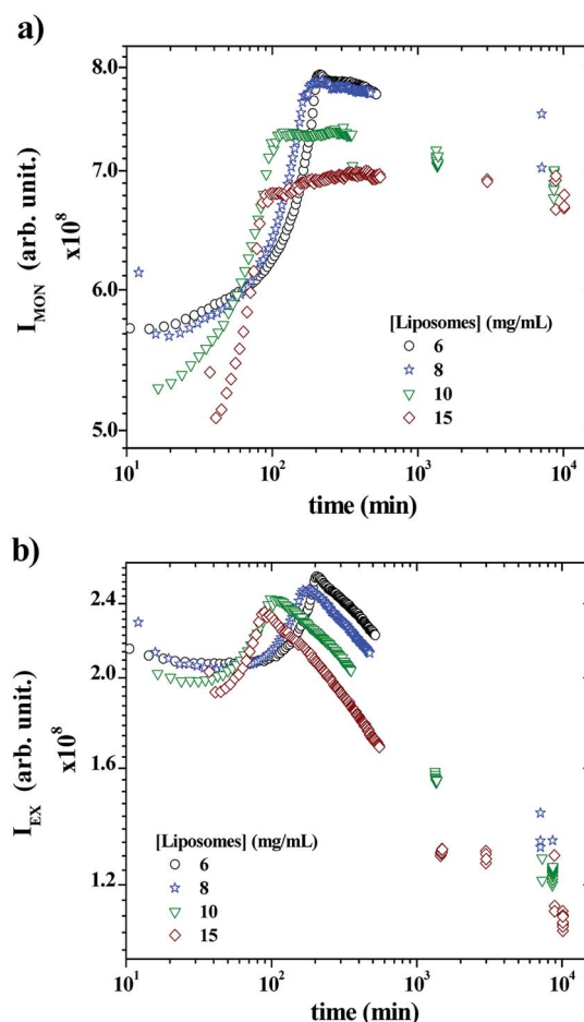
Fig. 5 (a) I_{\text{MON}} decay and (b) I_{\text{EX}} decay as a function of time obtained during the exchange of a mixture containing 3 \text{ mg mL}^{-1} P104 micelles with PyC 18 and liposomes suspensions with the following concentrations: 6, 8, 10 and 15 \text{ mg mL}^{-1} . The measurement temperature is 37^\circ\text{C} at a pH = 6.5.
