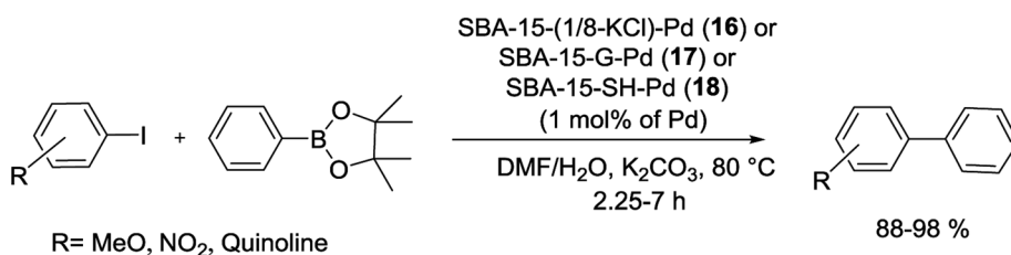
Scheme 20 S–M coupling reactions catalyzed by SBA-15-(1/8-KCl)-Pd (16), SBA-15-G-Pd (17) and SBA-15-SH-Pd (18).
