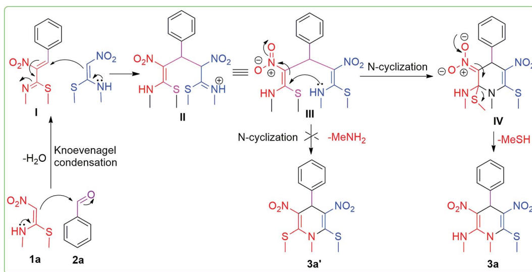
Scheme 2 Plausible reaction mechanism for the synthesis of N -methyl-1,4-DHPs.
