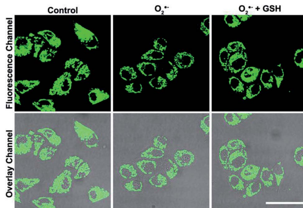
Fig. 5 Confocal fluorescence microscopic images of HeLa cells collected from different channels treated with S, N, O-CDs after the cells were stimulated by \text{O}_2^{\cdot-} in the absence and in the presence of GSH. Scale bar = 25 \mu\text{m} .
