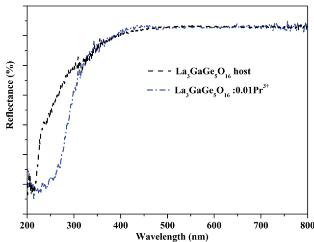
Fig. 2 (a) Diffuse reflectance spectra of pure \text{La}_3\text{GaGe}_5\text{O}_{16} and \text{La}_3\text{GaGe}_5\text{O}_{16}:\text{0.01Pr}^{3+} at room temperature.
