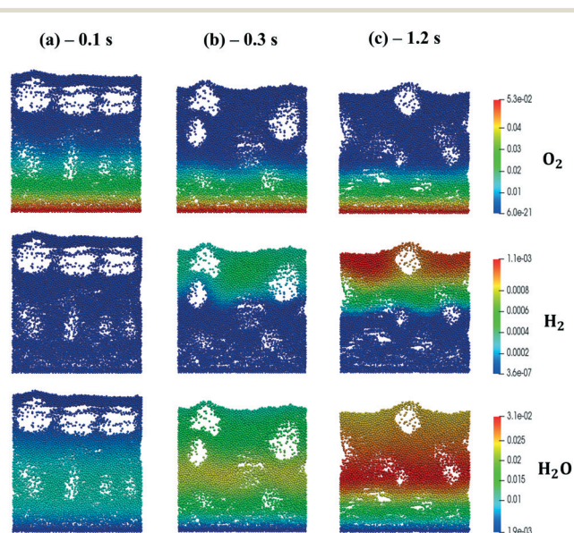
Fig. 4 Snapshot of the bubbling fluidized bed at the beginning of the simulation at t = 0.1 s (a), during the syngas production at t = 0.3 s (b) and the pseudo-steady state at t = 1.2 s (c), simulated with the operating conditions listed in Table 1 for the methane CPO. The catalytic bed is represented reporting each catalytic particle as a sphere. The catalytic pellets are mapped as a function of their O 2 , H 2 O and H 2 mass fraction. Particle-free regions represent the bubbles of gas.
