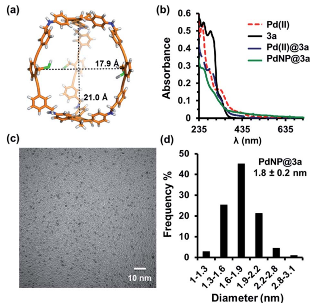
Fig. 1 (a) Calculated cavity size of fully extended cage 3a; (b) UV-vis absorption spectra of cage 3a and the palladium complexes in CH 2 Cl 2 ; (c) HRTEM micrographs (scale bar 10 nm) of PdNP@3a; (d) Size distribution of the PdNP@3a complex.
