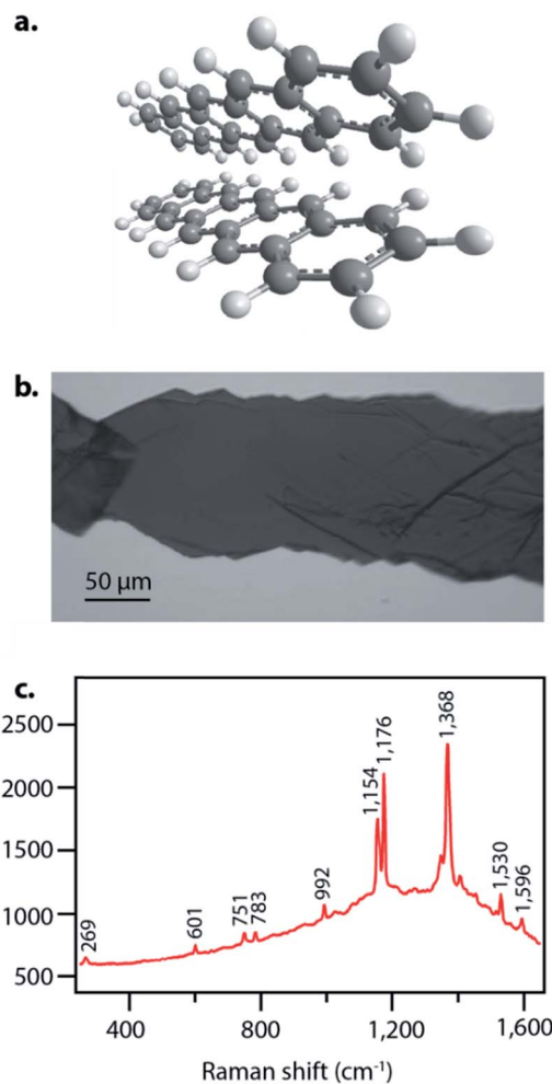
Fig. 1 Characterization of pentacene samples used for FSRS experiments. (a) Structure of pentacene in a herringbone structure characteristic of this crystalline solid. (b) Image of crystal used in the FSRS experiments, grown by physical vapor transport. (c) Spontaneous ground state Raman spectrum of crystalline pentacene at 633 nm excitation.
