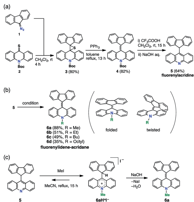
Fig. 2 Synthesis of FAs. (a) Barton–Kellogg reaction giving fluorenylacridine. (b) Installation of alkyl chains giving FA derivatives. Conditions: MeOTf, \text{K}_2\text{CO}_3 , MeCN, reflux, 15 h ( 6a ), EtOTf, \text{K}_2\text{CO}_3 , \text{CH}_2\text{Cl}_2 , rt, 15 h ( 6b ), BuOTf, \text{K}_2\text{CO}_3 , \text{CH}_2\text{Cl}_2 , rt, 15 h ( 6c ), and (i) OctylOH, TfOTf, EtOTf, \text{K}_2\text{CO}_3 , o -dichlorobenzene, 0 °C, 3 h, (ii) 5 , 50 °C, 17 h ( 6d ). (c) Equilibrium between 5 and an acridinium salt ( 6aH + I - ) in the methylation reaction.
