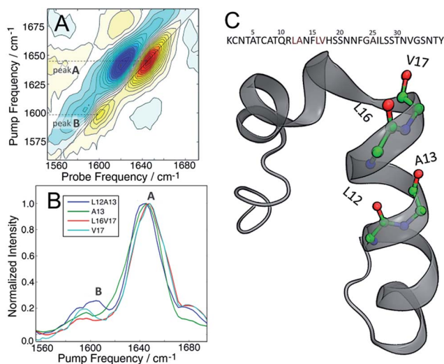
Fig. 2 (A) 2D IR spectrum of the L12A13 hIAPP in 100 mM SDS micelle solution. Unlabeled amides give rise to a broad band at 1650 cm -1 (peak A). A strong signal from the isotope labels is clearly seen at 1603 cm -1 (peak B). (B) Diagonal slices through the \nu = 1-2 band for all the studied isotope labels measured in SDS micelles. Only the L12A13 label (peak B) shows a strong positive coupling and a great intensity enhancement with respect to the corresponding single label (C) The sequence and NMR structure of human amylin in SDS micelles with the isotope labeling sites highlighted.
