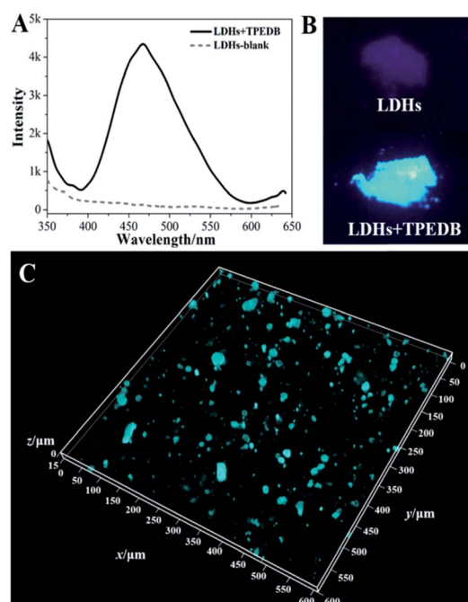
Fig. 3 (A) Fluorescence spectra and (B) photos under UV light of LDHs before and after the addition of TPEDB; (C) a 3D-representation of fluorescence confocal microscopy images ( 600 \times 600\ \mu\text{m}^2 ) of PE–5% LDH composite after staining with 100 \mu\text{M} TPEDB, the cyan colored patterns represent the stained LDH particles.
