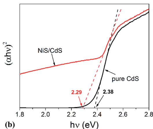
Fig. 6 (a) UV-visible absorption spectra of the pure CdS NWs, pure NiS nanostructures, and optimized NiS/CdS NWs. The insets display the digital photographs of the corresponding samples, which were dip-coated and naturally dried onto 1 \times 1 cm glass substrates. (b) The corresponding curves of (\alpha hv)^2 versus hv .
