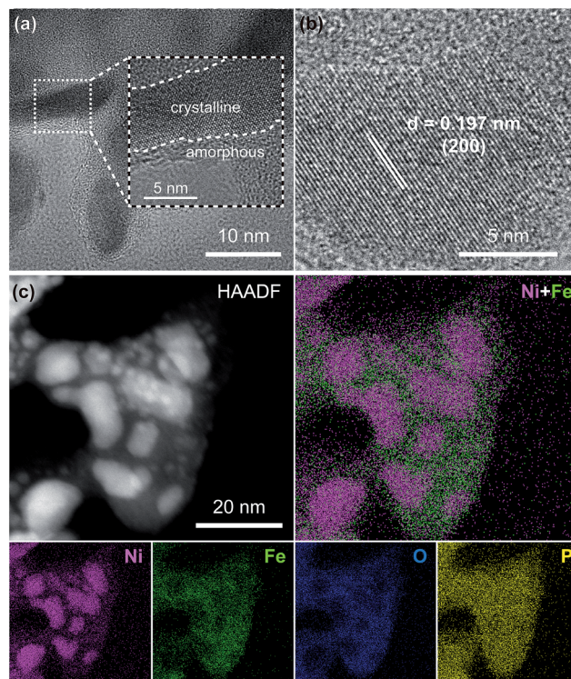
Fig. 2 (a) TEM image, (b) HRTEM image, (c) HAADF-STEM image and EDS elemental mapping images for the \text{Ni}_2\text{P}@ \text{FePO}_x sample.
