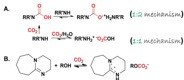
Scheme 3 (A) Proposed chemisorption of CO 2 by amine based substrates (primary and secondary, the general formula is given for the secondary for clarification) through the formation of RR'NH-CO 2 - +NH 2 -RR' and RR'NH 2 + -O 2 COH in the absence and presence of water, respectively. (B) The reversible reaction between an alcohol (ROH) and 1,8-diazabicyclo-[5.4.0]-undec-7-ene (DBU) in the presence of CO 2 .
