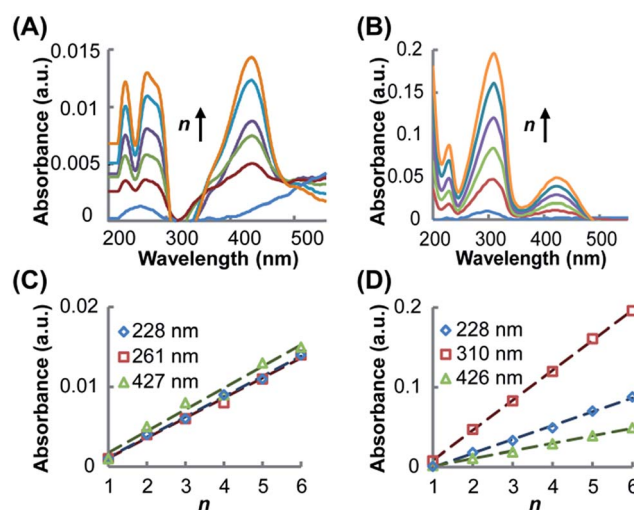
Fig. 2 UV-vis spectra of (\text{Rh}_2L_s)_n@Au (A) and (\text{Rh}_2L_l)_n@Au (B), showing the increase of band intensity with increasing the number of layers n from 1 to 6 (from bottom to top). Linear relationships between the absorbance and n for (\text{Rh}_2L_s)_n@Au (C) and (\text{Rh}_2L_l)_n@Au (D), determined from the three major absorption bands in the spectra.
