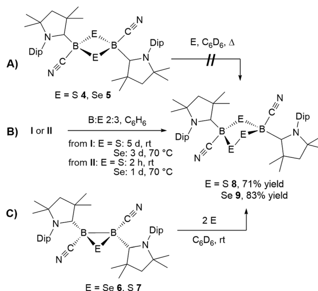
Scheme 7 Unsuccessful ring-expansion of 1,3-dichalcogen-2,4-diboretanes (A) and successful syntheses of 1,2,4-trichalcogena-3,5-diborolanes from I or II (B) and by ring-expansion of 1,2,3-trichalcogenadiboriranes (C).
