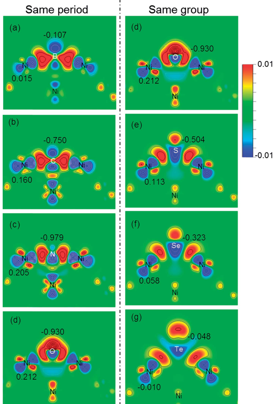
Fig. 4 The charge density difference plots (ranging from -0.01 to 0.01 \text{ e}^-3 ) that contain the X–Ni bond and the corresponding Bader charge ( Q/e ) in the X/Ni(100) systems: (a) B/Ni(100); (b) C/Ni(100); (c) N/Ni(100); (d) O/Ni(100); (e) S/Ni(100); (f) Se/Ni(100); (g) Te/Ni(100).
