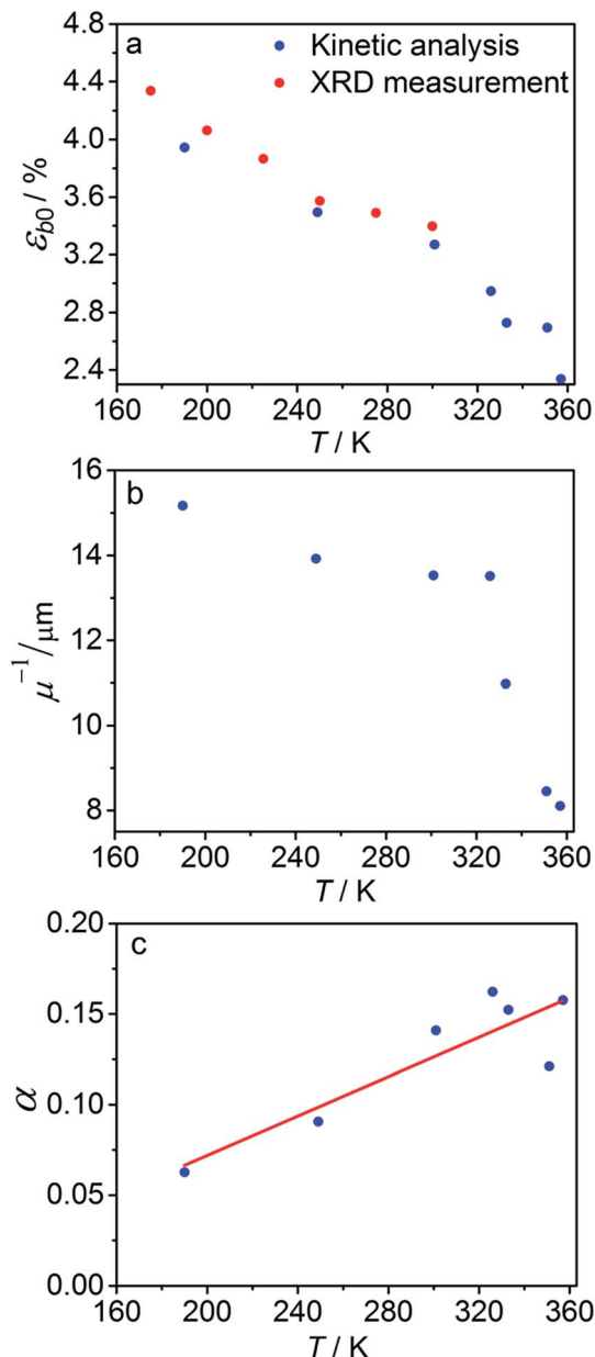
Fig. 7 Temperature dependence of the maximum deformation \varepsilon_{b0} (a), characteristic penetration depth (reciprocal of the absorption coefficient \mu ) (b), and quantum yield \alpha (c) obtained using the simple kinetic model given by eqn (11) that accounts only for the dependence on the temperature and disregards the variation with the composition.
