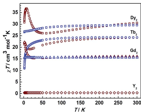
Fig. 5 Temperature dependence of the \chi_M T values at 1000\text{ Oe} for compounds 1Ln and 2Ln . The blue and brown symbols correspond to neutral and radical compounds, respectively.
