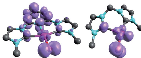
Fig. 11 Spin densities of NHC complex 31^{\text{PdO}} (left side) and 18^{\text{PdO}} (right side) in the triplet states.
