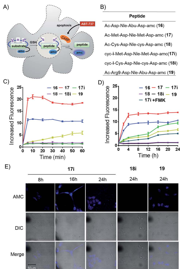
Fig. 5 (A) Schematic illustration of the AMC release assay. (B) Peptides used for the AMC release assay. (C) AMC release efficiency of peptides 16–19 (5 \mu M) treated with caspase-3 protein for 1 h and monitored at 5 minute intervals. (D) Time-dependent release of AMC of peptides 16–19 (5 \mu M) treated with U2OS cell lysates in the absence and presence of caspase inhibitor FMK (100 \mu M) for 24 h. (E) Confocal microscopy images of U2OS cells after treatment with peptides 17i , 18i and 19 at 100 \mu M for 4 h, followed by incubation with GSH at 10 mM for 8, 16, or 24 h and then treatment with the apoptotic inducer ABT-737 (10 \mu M) for 1 h.
