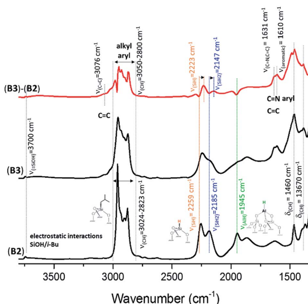
Fig. 3 FT-IR spectra of \text{Al}^i\text{H}@KCC-1700 ( B2 ) and B3 formed after reaction with HG-II . Subtraction ( B3 – B2 ) is given in red.
