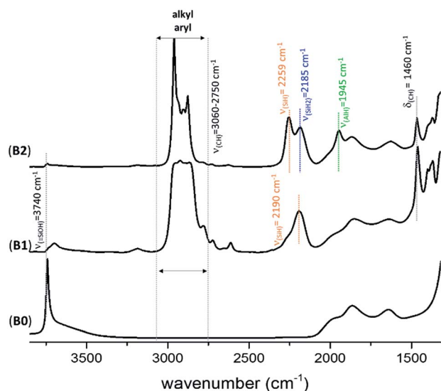
Fig. 2 FT-IR spectra of KCC-1700 ( B0 ), \text{Al}^i\text{Bu}@KCC-1700 ( B1 ) and \text{Al}^i\text{H}@KCC-1700 ( B2 ).
