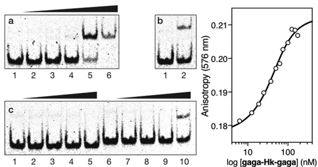
Fig. 4 Left: EMSA results for gaga-Hk-gaga . Panel (a), lanes 1–6: [gaga-Hk-gaga] = 0, 300, 500, 700, 1000, and 1500 nM with 75 nM CTC·AT·GAG . Panel (b), lanes 1–2: [gaga-Hk-gaga] = 0 and 1000 nM with 75 nM cat·AT·GAG . Panel (c), lanes 1–5: [gaga-Hk-gaga] = 0, 300, 500, 700, and 1000 nM with 75 nM cat·AT·cgc . Panel (c), lanes 6–10: [gaga-Hk-gaga] = 0, 300, 500, 700, and 1000 nM with 75 nM CTC·gc·GAG . Oligonucleotide sequences (only one strand shown): CTC·AT·GAG : 5'-GAG CTCTC AATT GAGAG CGCG-3'; cat·AT·GAG : 5'-CGC GTCAT AATT GAGAG CGC-3'; cat·AT·cgc : 5'-CGC GTCAT AATT CGCGA CGC-3'; CTC·gc·GAG : 5'-GGTT CTCTC GACC GAGAG TTGG-3'. Experimental conditions are as indicated in the caption of Fig. 2. Right: Fluorescence anisotropy titration of a 25 nM solution of TMR- CTC·AT·GAG with increasing concentrations of gaga-Hk-gaga and best fit to a 1 : 1 binding model. Data are the mean of three titrations.
