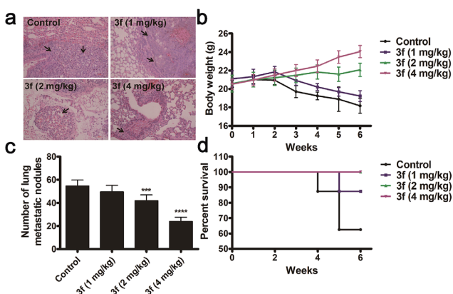
Fig. 6 Compound 3f inhibits the lung metastasis of MDA-MB-231 cells in mice. (a) Representative images of lung metastasis from mice in different groups ( n = 8 ) (scale bar: 100 \mu\text{m} ). (b) Numbers of lung metastatic nodules from mice in different groups. (c) Body weight. (d) Survival rate. n = 5 in the control group; n = 7 in the 3f (1 mg kg -1 ) group; n = 8 in the other 2 groups. Values are means \pm S.D. *** P < 0.001 , **** P < 0.0001 vs. the control group.
