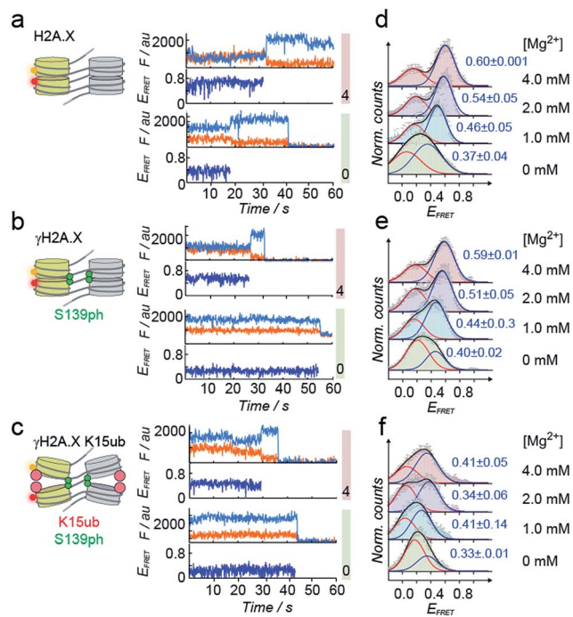
Fig. 4 H2A.X K15ub inhibits tetranucleosome compaction. (a) Single-molecule traces (donor: orange, acceptor: red, FRET: blue) for H2A.X at 0 mM \text{Mg}^{2+} (bottom), 4 mM \text{Mg}^{2+} (top) until donor or acceptor photobleaching. (b) FRET traces for \gamma H2A.X, same conditions as in (a). In the scheme, the green sphere indicates S139 phosphorylation. (c) FRET traces for \gamma H2A.X K15ub, same conditions as in (a). The red sphere indicates H2AK15 ubiquitylation. (d) FRET populations observed for H2A.X at the indicated \text{Mg}^{2+} concentrations. The number indicates the center of the high-FRET population ( \pm s.d. from 2 to 3 independent experiments). For the number of replicates and Gaussian fit parameters, see Table S2.† (e) FRET populations observed for \gamma H2A.X at the indicated \text{Mg}^{2+} concentrations. (f) FRET populations observed for \gamma H2A.X K15ub at the indicated \text{Mg}^{2+} concentrations.
