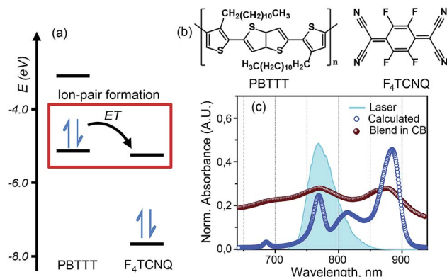
Fig. 1 PBTTT/ F_4TCNQ : a model system for the ion-pair in p-doped organic semiconductors. (a) Unperturbed energy diagram depicting the electronic states of PBTTT and F_4TCNQ , which are involved in the formation of the ion-pair. Electron transfer (ET) from PBTTT to F_4TCNQ is favored by the sizable energy offset between the ionization energy (IE) of PBTTT ( -5.1 eV) and the electron affinity (EA) of F_4TCNQ ( -5.2 eV). The values of the IE and EA of F_4TCNQ and PBTTT are used from literature report. 16 (b) Chemical structures of the polymer PBTTT and the dopant, F_4TCNQ , used in this study. (c) Experimental (brown spheres) and calculated (blue circles) absorption spectra of the PBTTT^+F_4TCNQ^- ion-pair at room temperature. The vibronic features in the experimental absorption spectrum in chlorobenzene are diagnostic for the F_4TCNQ anion ( D_0 \rightarrow D_1 ). The blue filled curve represents the laser spectrum used in the two-dimensional electronic spectroscopic measurements which covers the polaron peak, P_2 of PBTTT at 815 nm ( \sim 12\,250 cm^{-1} ) as well as the second vibronic feature at 769 nm ( \sim 13\,000 cm^{-1} ) corresponding to the F_4TCNQ anion.
