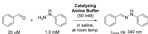
Scheme 1 Model reaction between benzaldehyde and phenylhydrazine.
