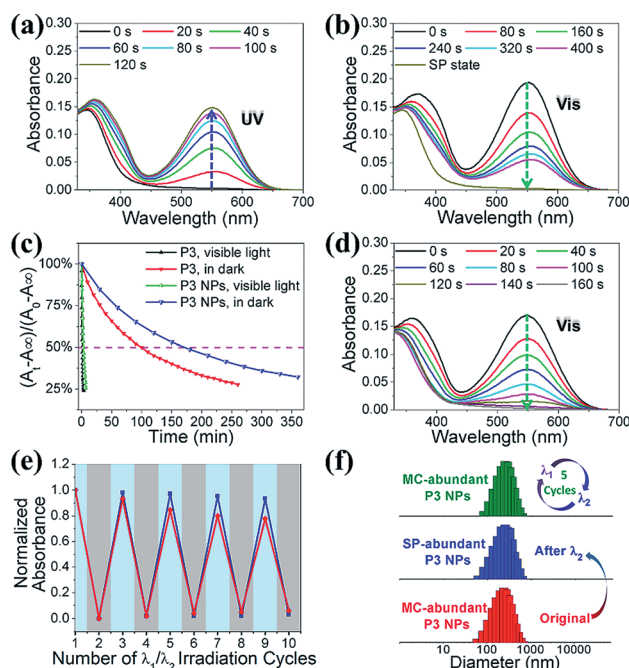
Fig. 3 Absorption spectra of the P3 NPs under (a) UV light ( \lambda_1 = 365 nm, 2 \text{ mW cm}^{-2} , 0–120 s) irradiation and (b) visible light ( \lambda_2 = 520 nm, 20 \text{ mW cm}^{-2} , 0–400 s) irradiation. (c) MC-SP isomerization kinetics of P3 and the P3 NPs in the dark or under visible light. A_0 , A_\infty and A_t are the absorption intensities at 549 nm, measured at the beginning, at the end and at the time of reaction, respectively. (d) Absorption spectra of the P3 NPs under visible light ( \lambda_2 > 500 nm, 250 \text{ mW cm}^{-2} , 0–160 s) irradiation. (e) Photoswitching cycles of the P3 NPs under irradiation by alternating 365 nm UV light and 520 nm visible light. Absorption intensities were monitored at 549 nm. The red and blue lines denote the measurements in the air-saturated and degassed solutions, respectively. (f) Comparison of hydrodynamic diameters of the P3 NPs before and after different irradiation treatments.
