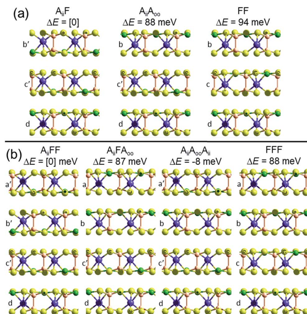
Fig. 2 Multilayer PBE-D3 optimized structures and relative energies \Delta E per cell, made based on the observed crystal structure of ferroelectric \text{CuInP}_2\text{S}_6 , for (a) trilayers and (b) tetralayers, labelled and cross-sectioned as in Fig. 1. P–brown, S–yellow, Cu–green, In–purple.
