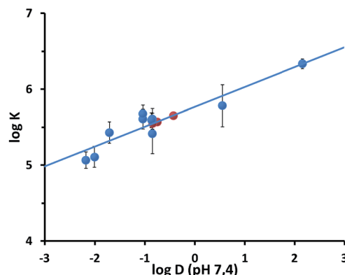
Fig. 5 Plot of the \log K vs. \log D (pH = 7.4) values relative to the binding of the luminescent analytes 8 – 13 and 17 – 19 to S1-AuNP. The lines represent the linear fit of the data ( R = 0.885 ). Red circles report the affinity values estimated for substrates 1 , 14 and 15 on the basis of their \log D values and the fitting parameters. The error bars reported represent the confidence intervals ( 3\sigma ) calculated from standard deviations reported in Table 1.
