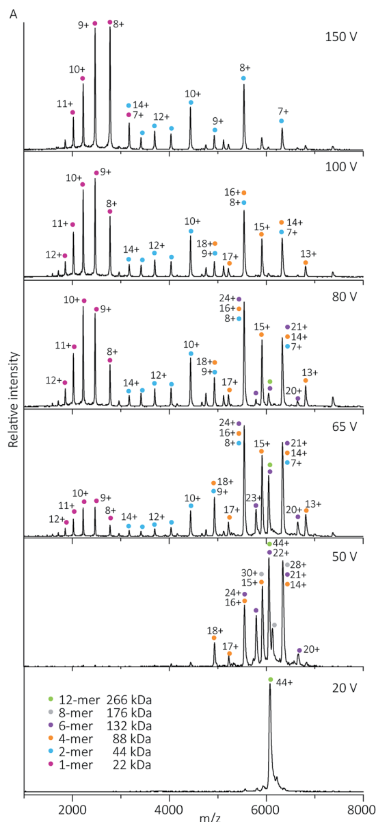
B CID breakdown pathway of peroxidoredoxin
