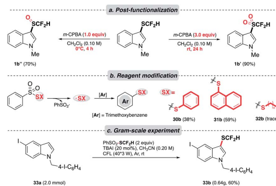
Scheme 4 Application. (a) Controlled oxidation of thioethers to corresponding sulfoxides and sulfones; (b) modified reagents to afford arylation products; (c) scaled-up experiments.
