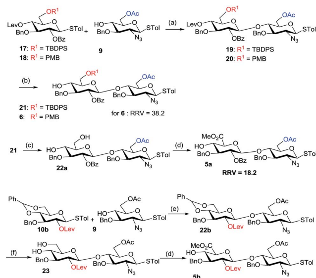
Scheme 2 Reaction conditions: (a) NIS, TfOH, \text{CH}_2\text{Cl}_2 , AW 300 MS, -45\text{ }^\circ\text{C} to -30\text{ }^\circ\text{C} , 2 h; 19 : 76%, 20 : 73%; (b) \text{NH}_2\text{NH}_2 \cdot \text{H}_2\text{O} , AcOH : Py (2 : 3), rt, 2 h; 6 : 90%, 21 : 88% (c) HF-Py, Py, 0\text{ }^\circ\text{C} to rt, 12 h, 81%; (d) (i) BAIB, TEMPO, \text{CH}_2\text{Cl}_2 : \text{H}_2\text{O} (2 : 1), 0\text{ }^\circ\text{C} to rt, 2 h; (ii) Mel, \text{KHCO}_3 , DMF, rt, 4 h, 0\text{ }^\circ\text{C} to rt, 5a : 63%, 5b : 61% (two steps); (e) (i) NIS, TMSOTf, \text{CH}_2\text{Cl}_2 , AW 300 MS, -20\text{ }^\circ\text{C} to 0\text{ }^\circ\text{C} , 15 min; 22b : 89%. (f) 80% AcOH, 70\text{ }^\circ\text{C} , 3 h; 23 : 79%.
