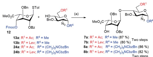
Scheme 3 Reaction conditions: (a) (i) NIS, TfOH, \text{CH}_2\text{Cl}_2 , AW 300 MS, -60\text{ }^\circ\text{C} to -30\text{ }^\circ\text{C} , 1 h; (ii) \text{Et}_3\text{N} , rt, 1 h.
